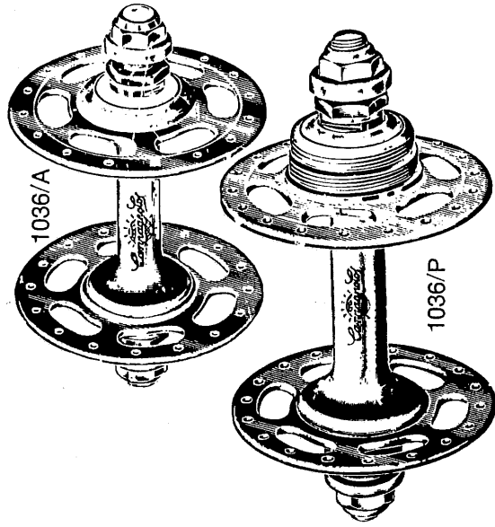
1036 RECORD LARGE FLANGE SOLID SPINDLE TRACK HUBS
