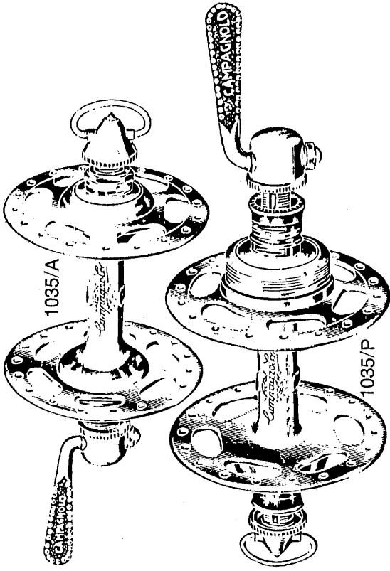
1035 RECORD LARGE FLANGE CAMPAGNOLO QUICK RELEASE ROAD HUBS
