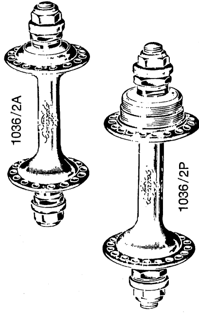
1036/2 RECORD SMALL FLANGE SOLID SPINDLE TRACK HUBS
