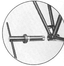
C-358 RIGHT BOTTOM BRACKET CUP TURNER
